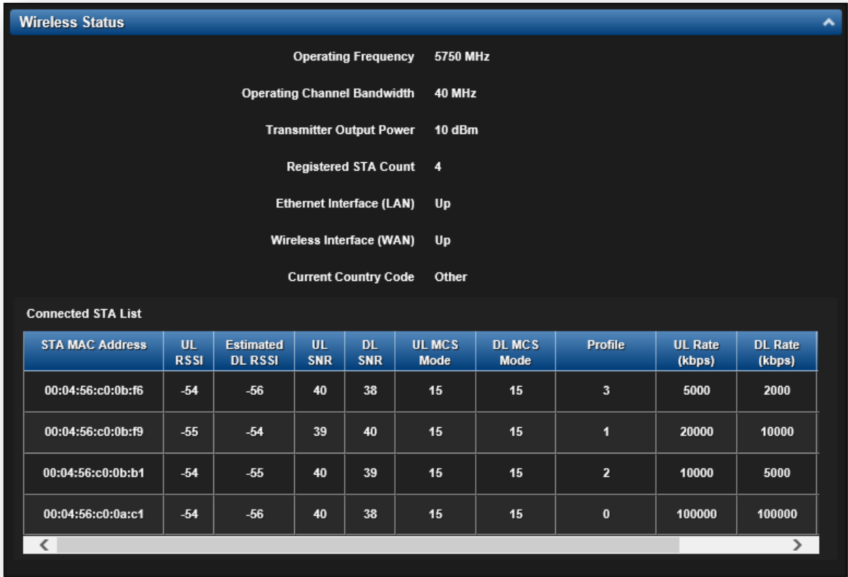
Figure 29 AP Wireless Status page
