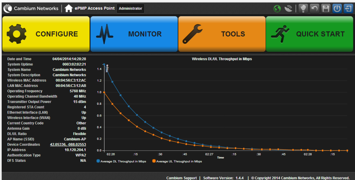
Figure 13 GUI dashboard
